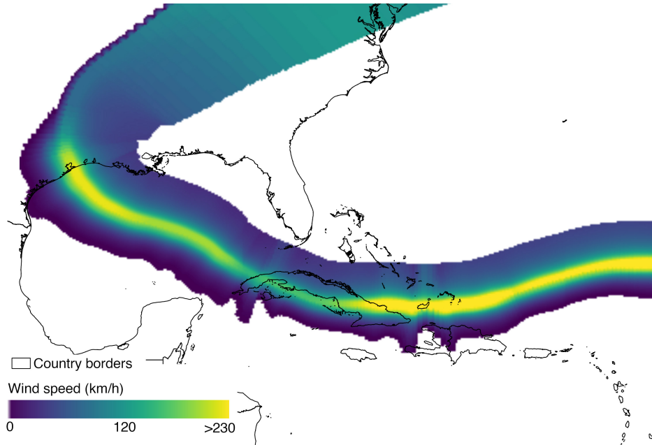
Figure 1: Wind field model for Hurricane Ike, 2008.
